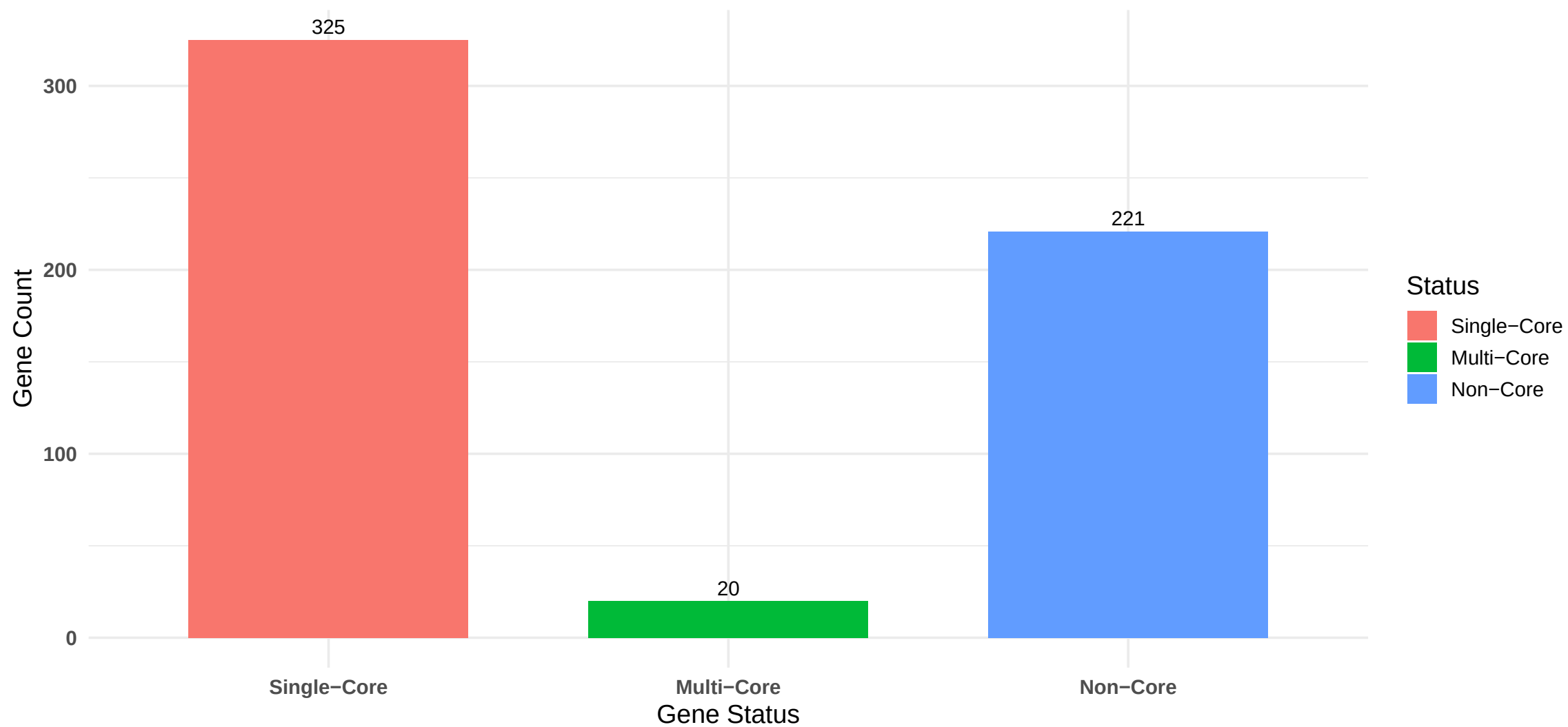
C. albicans DEGs by Orthogroup gene classification
