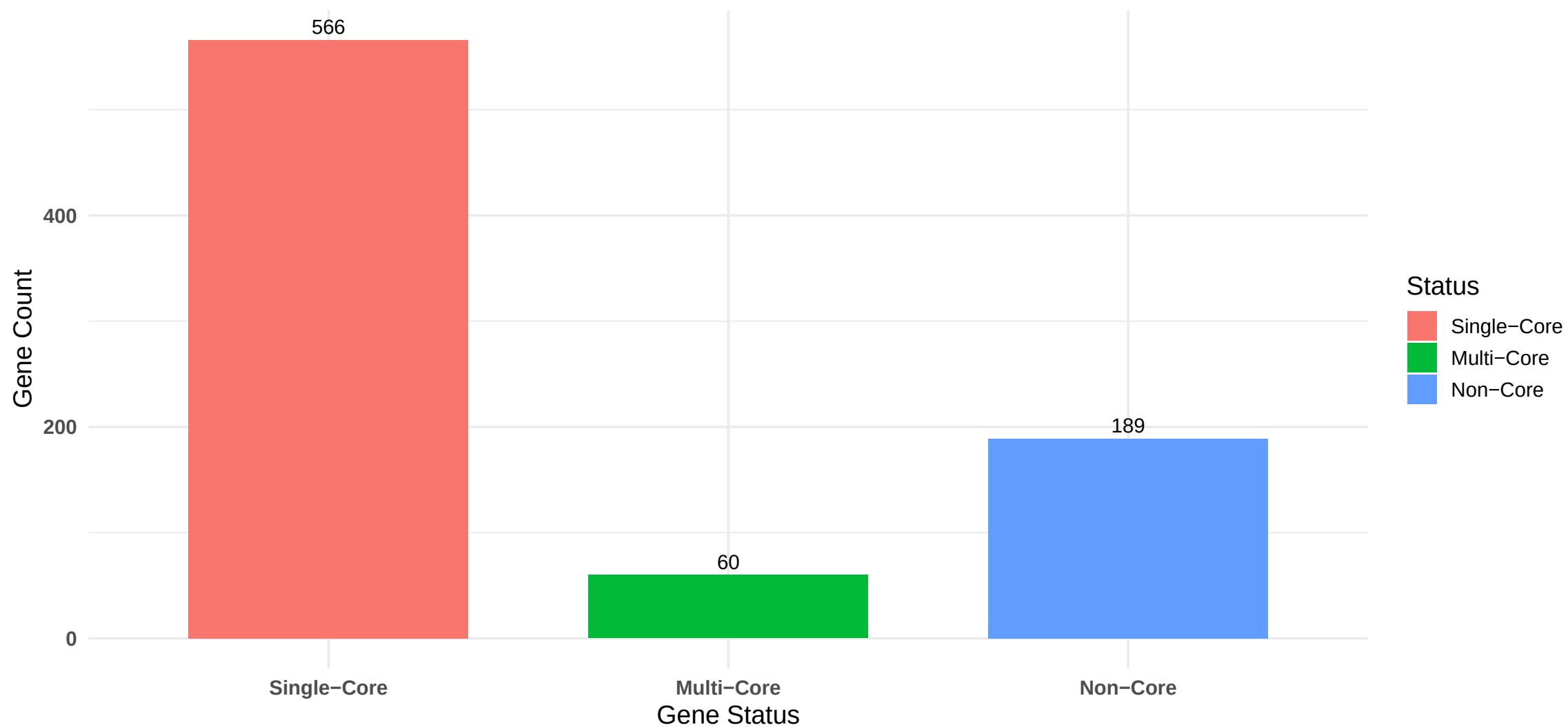
C. glabrata DEGs by Orthogroup gene classification
