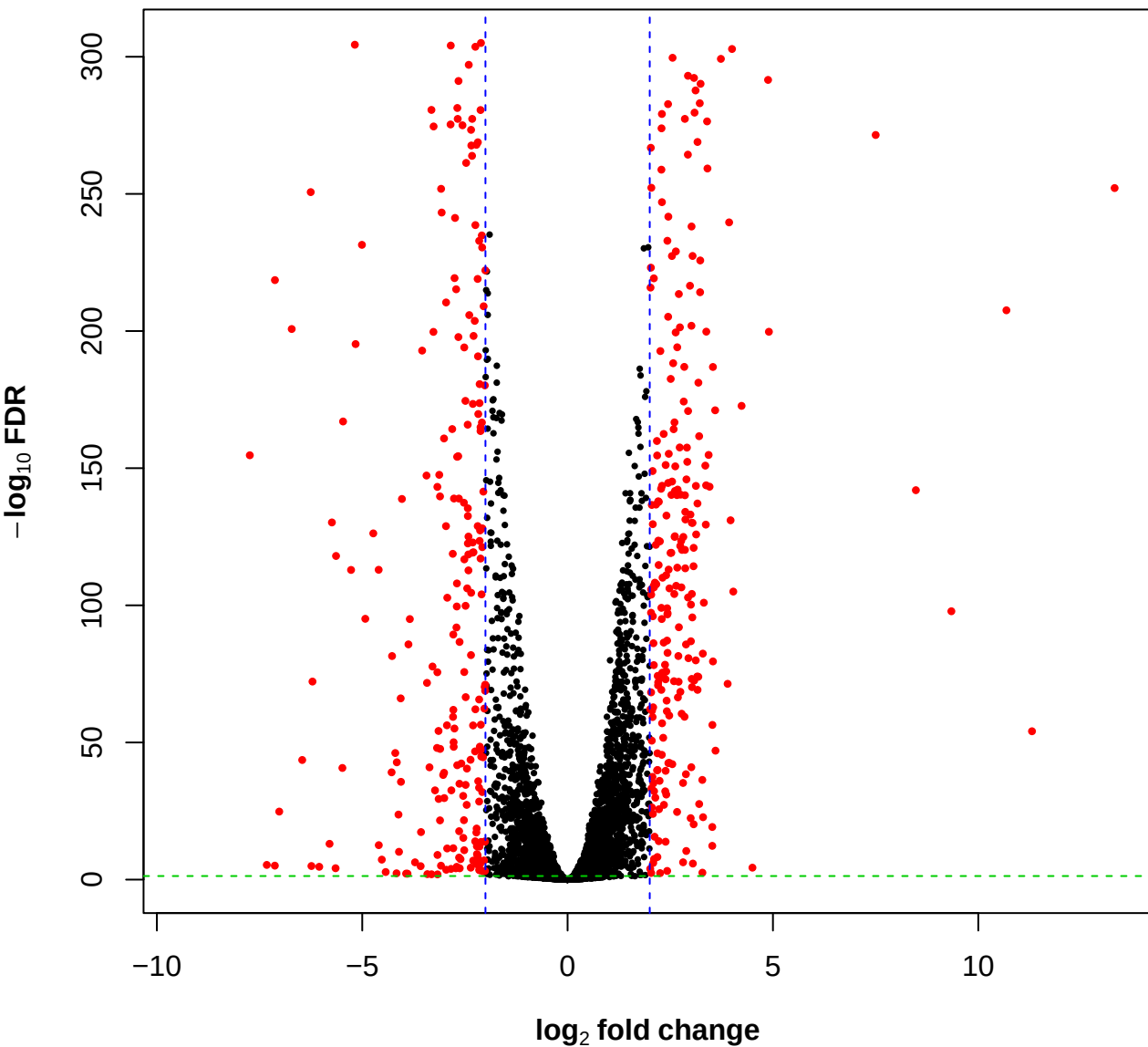
Volcano Plot – Calb t0000 vs t0060
