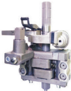
Sr No.: 4195-A : HYD. LIFT PUMP ASSLY. ( CURVE TYPE LEVER ) WITH HEX TYPE RELIEF VALVE Ref. No.: 4200076M91
