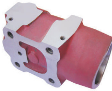
Sr No.: 4136 : HYD. LIFT RAM CYLINDER MF. { 85.50 MM } Ref. No.: 1671082M1 / 897594M2
