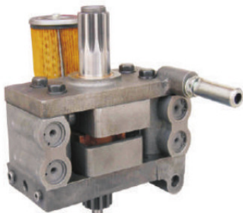
Sr No.: 5028 : HYD. PUMP ASSLY. SWARAJ Ref. No.: P-281700
