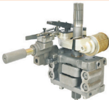
Sr No.: 4169 : HYD. LIFT PUMP ASSLY. WITH PRESSURE CONTROL UNIT MF-245/240
