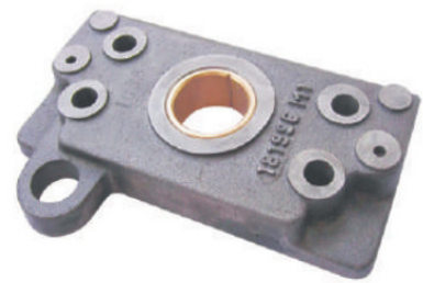
Sr No.: 4062 : HYD. PUMP PLATE ( SMALL ) FRONT WITH BUSH & SCREW MF-1035 Ref. No.: 181996M1 / 182006M91
