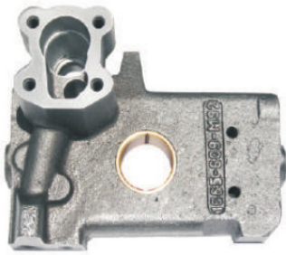
Sr No.: 4145 : HYD. PUMP PLATE ( BIG ) REAR WITH BUSH THREAD SIZE 3/8" BSW MF-285 Ref. No.: 1665610M1
