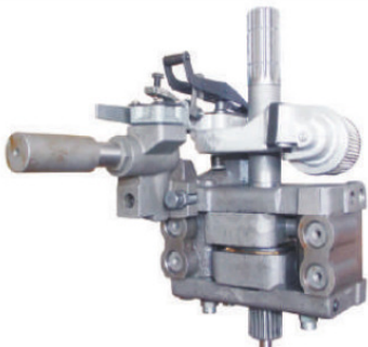
Sr No.: 4191 : HYD. LIFT PUMP ASSLY. WITH PRESSURE CONTROL UNIT (21 SPLINES) MARK III (CURVE TYPE LEVER) Ref. No.: 3773700M92
