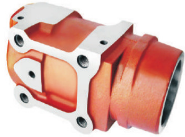
Sr No.: 4020 : HYD. LIFT RAM CYLINDER MF-245 ( 79 MM ) Ref. No.: 897560M3
