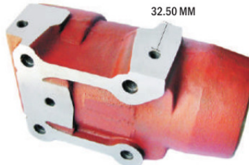
Sr No.: 4235-A : HYD. RAM CYLINDER IMT (76 MM) ( M M THREAD ) (SIDE HOLE 32.50 MM ) Ref. No.:
