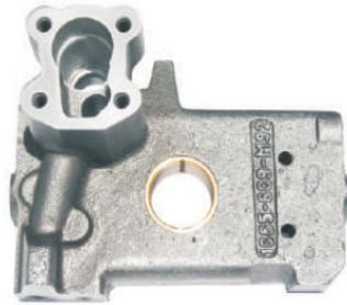
Sr No.: 4092 : HYD. PUMP PLATE ( BIG ) REAR WITH BUSH RELIEF VALVE THREAD 9/16 UNF MF-245 Ref. No.: 1665609M92
