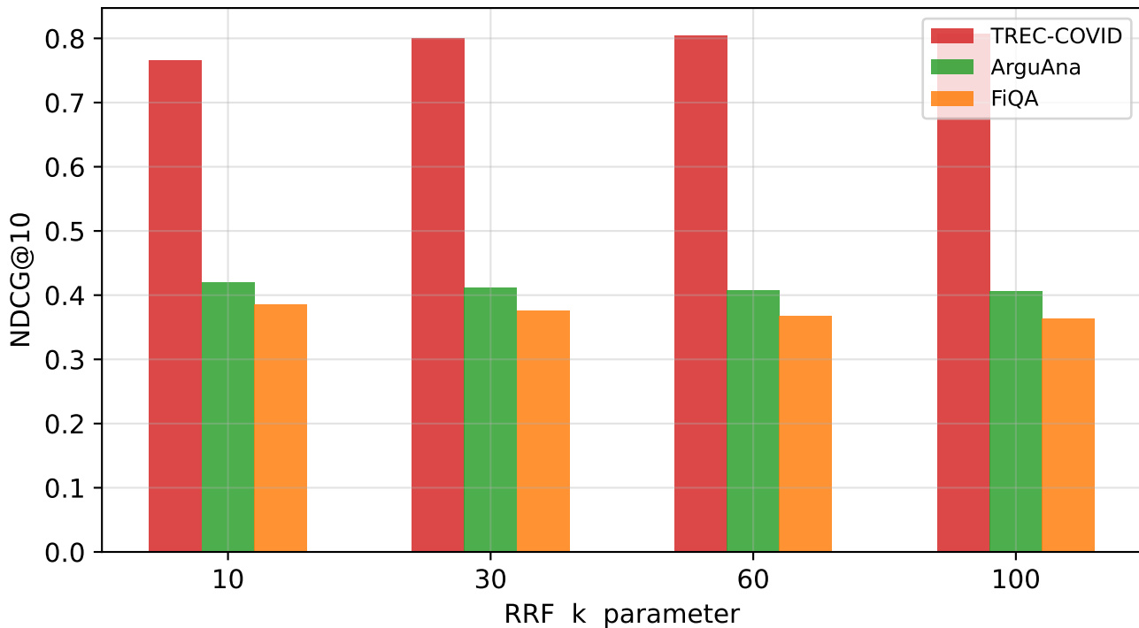
Strategy B — RRF Sensitivity to k
