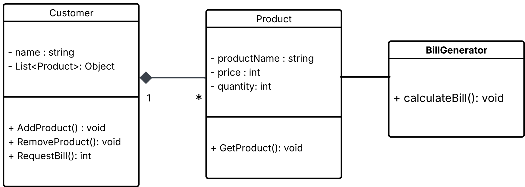
Fig: Class Diagram
