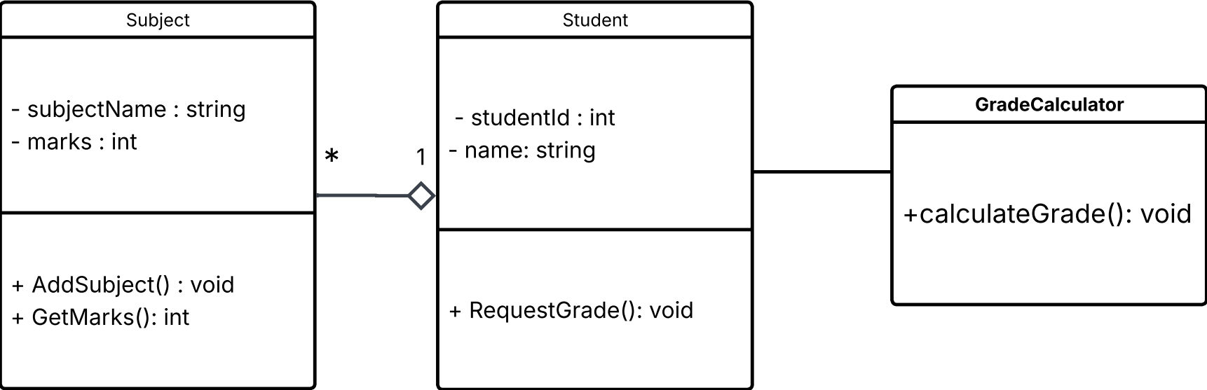
Fig: Class Diagram
