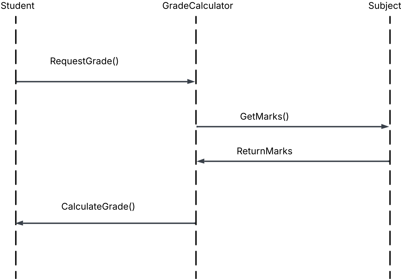
Fig: Sequence Diagram
