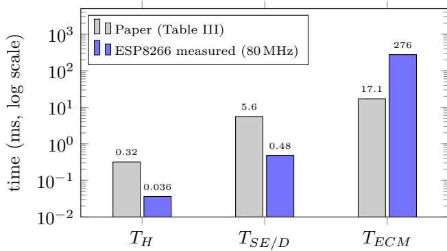
Fig. 1. Assumed versus measured per-operation time on the ESP8266 ( T_{SE/D} is aes_big GCM; aes_ct gives 1.15 ms).
