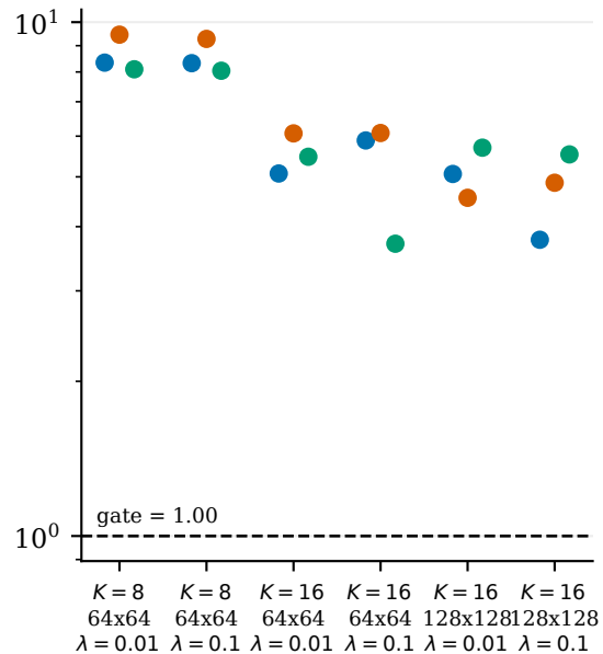
90th percentile |L^+ \rho/\rho|
