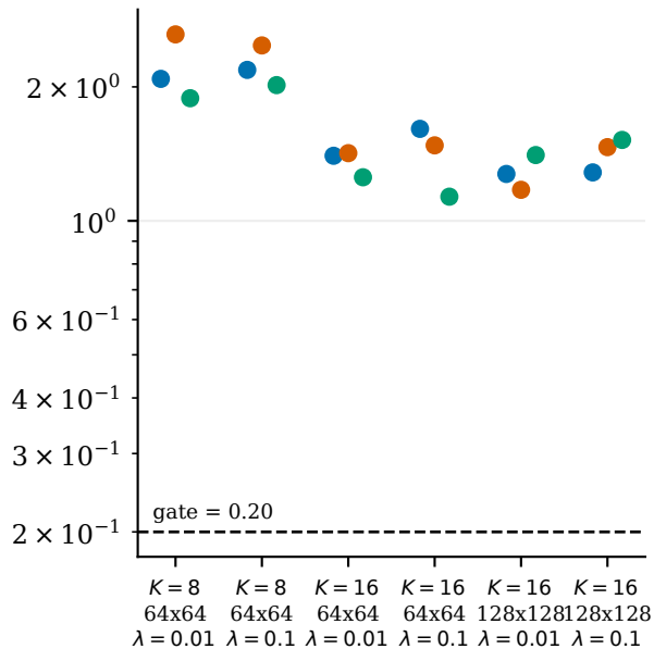
median |L^+ \rho/\rho|
