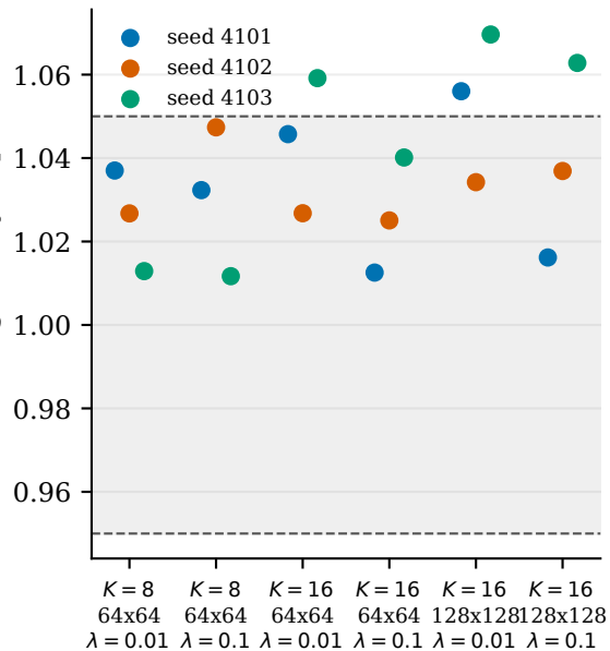
Gibbs log-density slope
