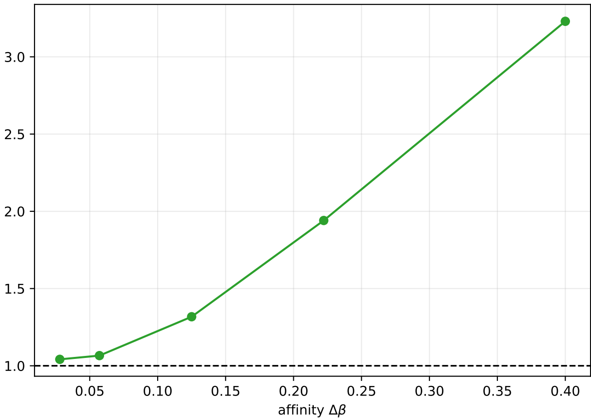
Gaussian FT ratio at t = 640
