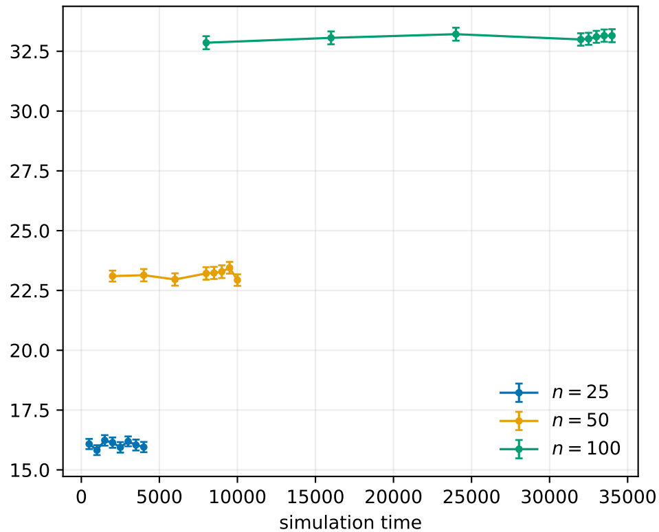
instantaneous ensemble mean M
