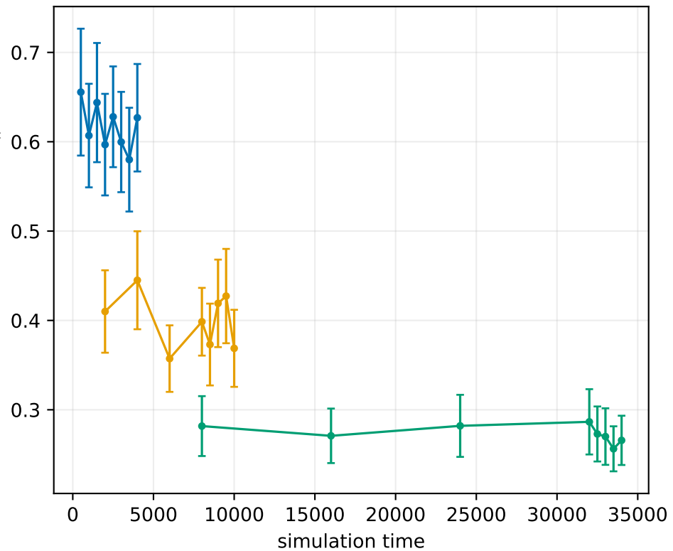
instantaneous free-end \langle I_n \rangle
