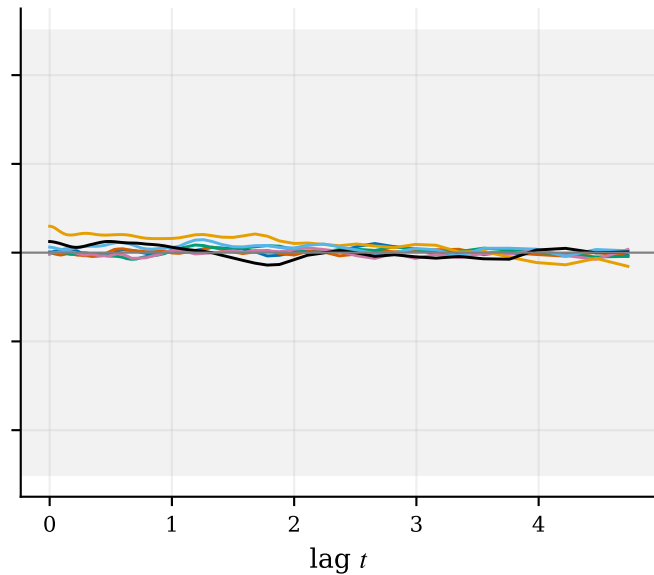
Equal temperature: (T_1, T_3) = (5, 5)
