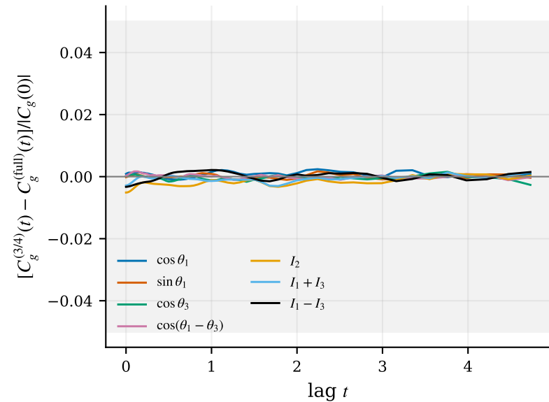
Driven: (T_1, T_3) = (2, 8)
