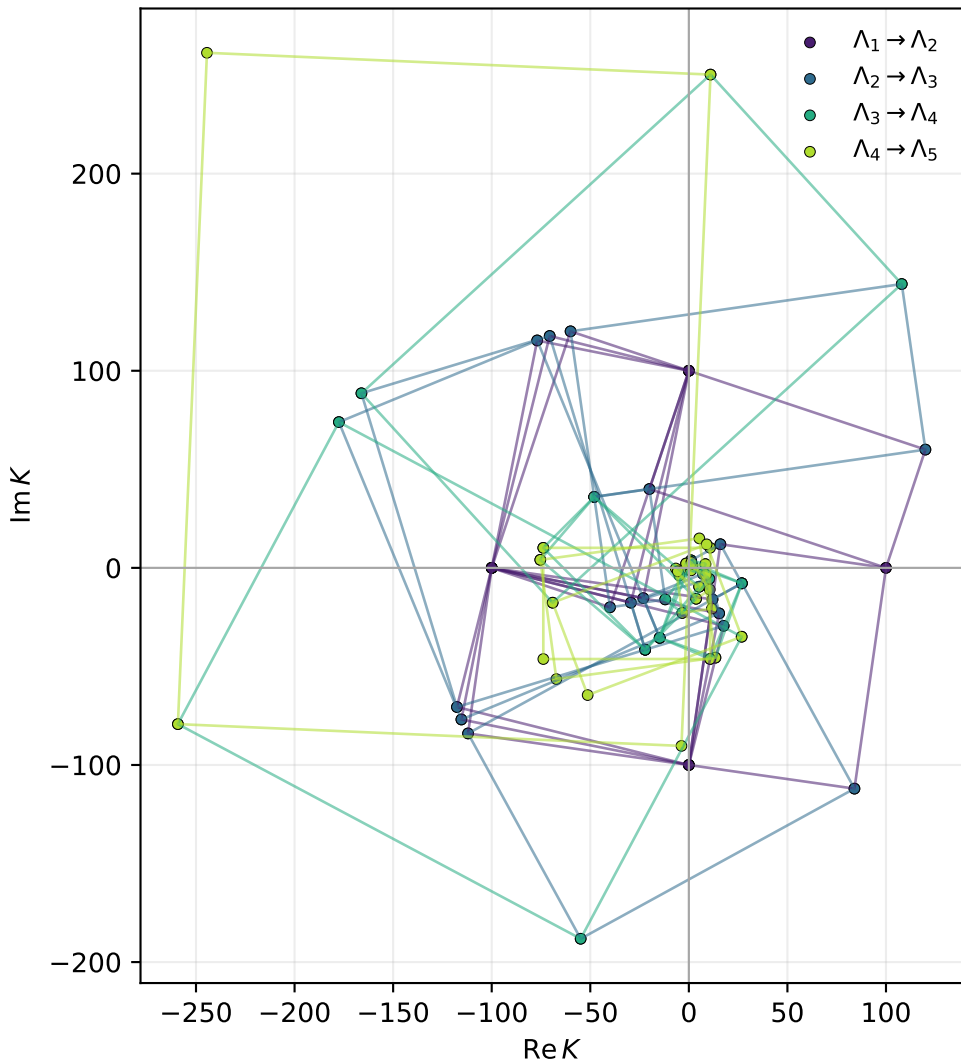
CKSTT resonant-family embedding, first five generations
