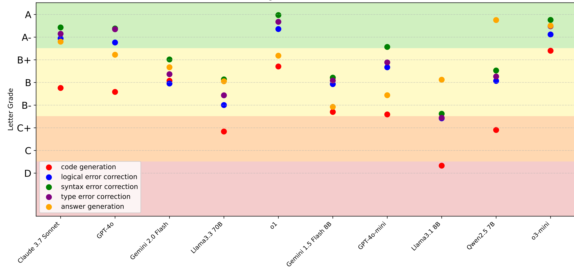
LLM Weighted Grades Across Tasks
