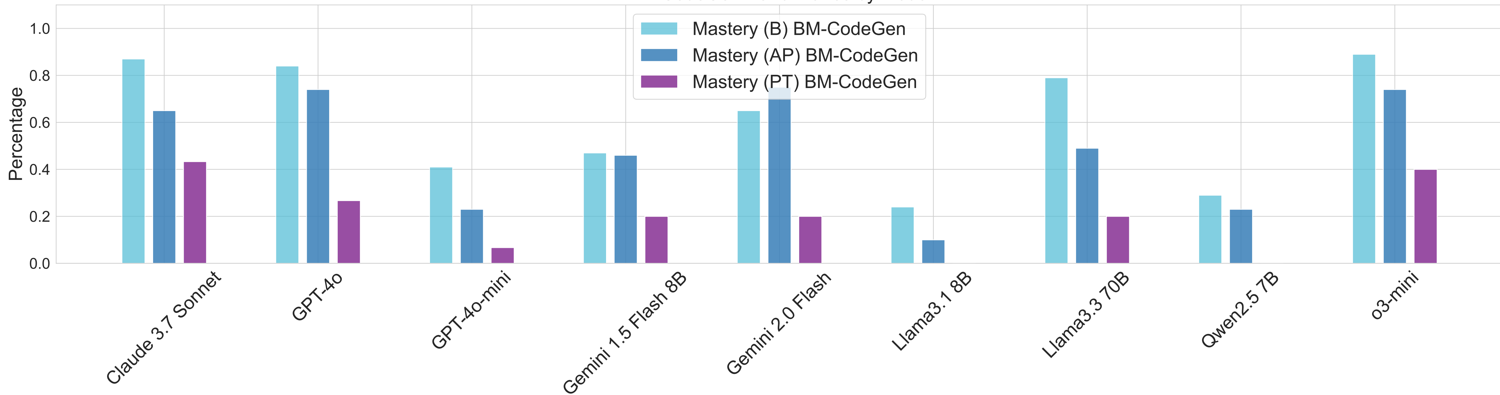
BM-CodeGen Performance by Model
