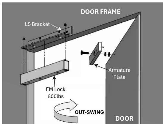
Mounting on single out-swing door
