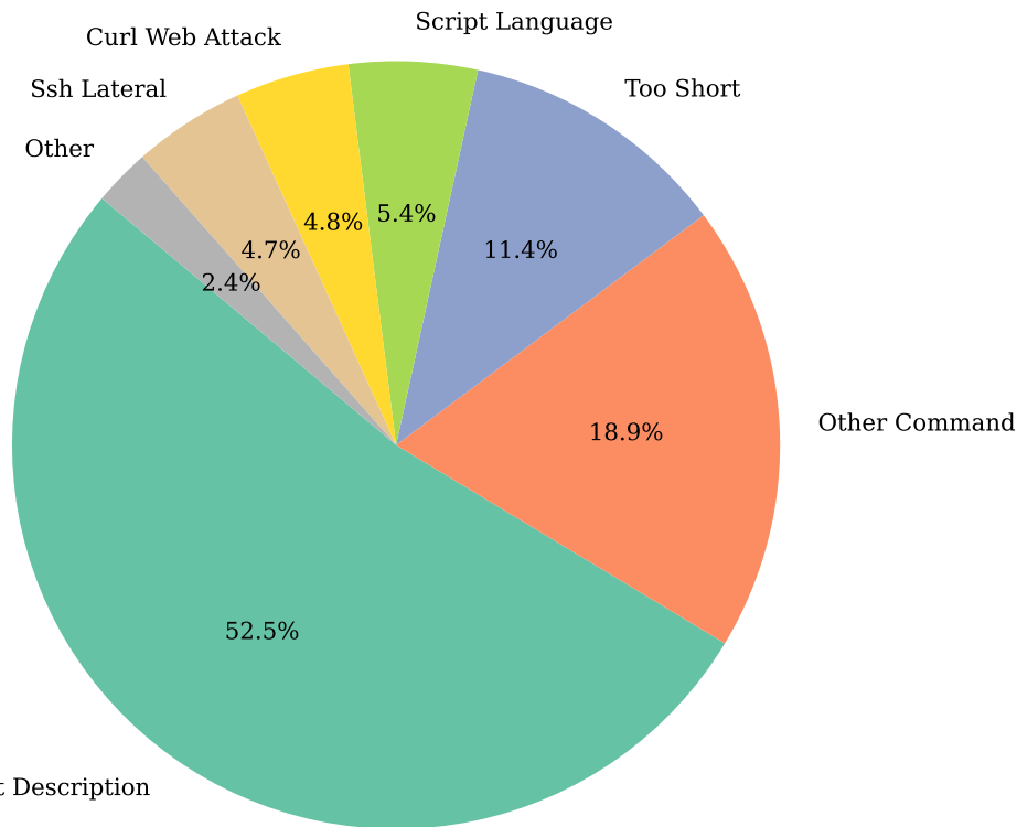
False Negative Reasons (n=1294)
