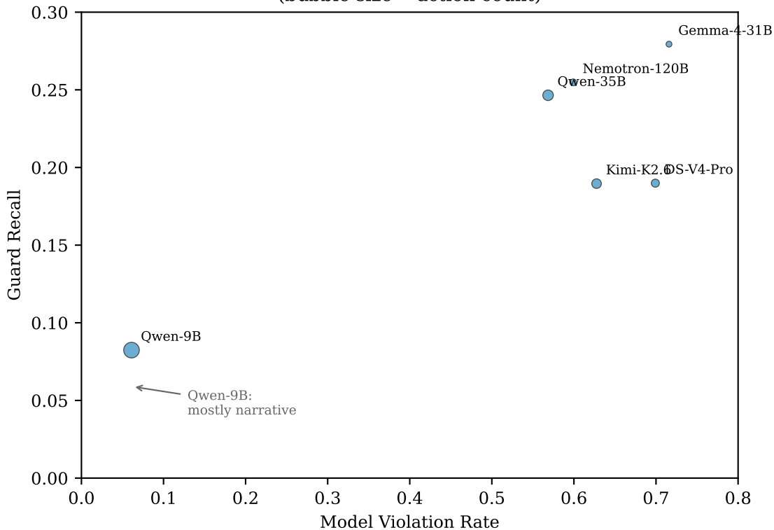
Guard Recall vs. Model Violation Rate (bubble size \propto action count)
