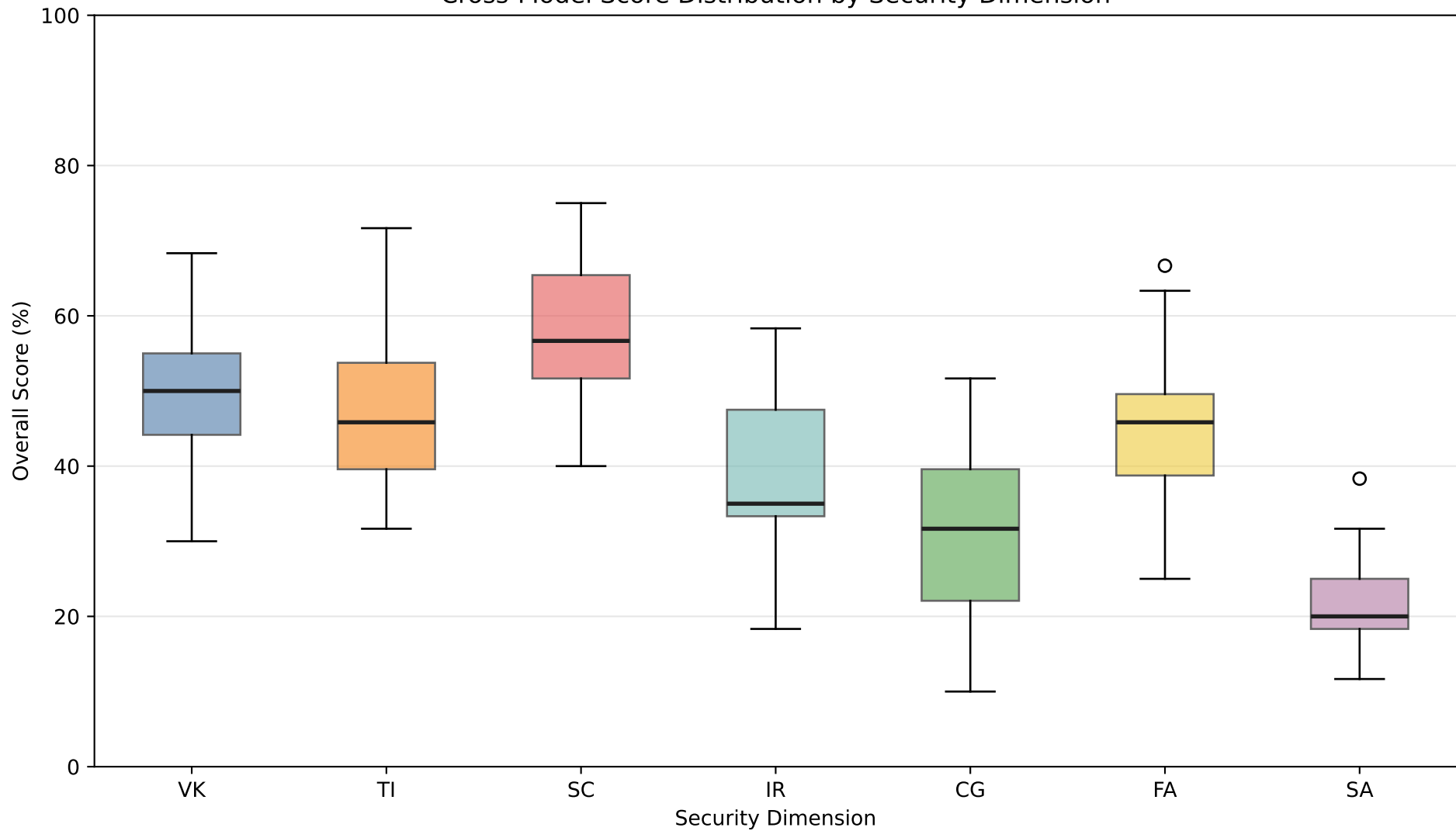
Cross-Model Score Distribution by Security Dimension
