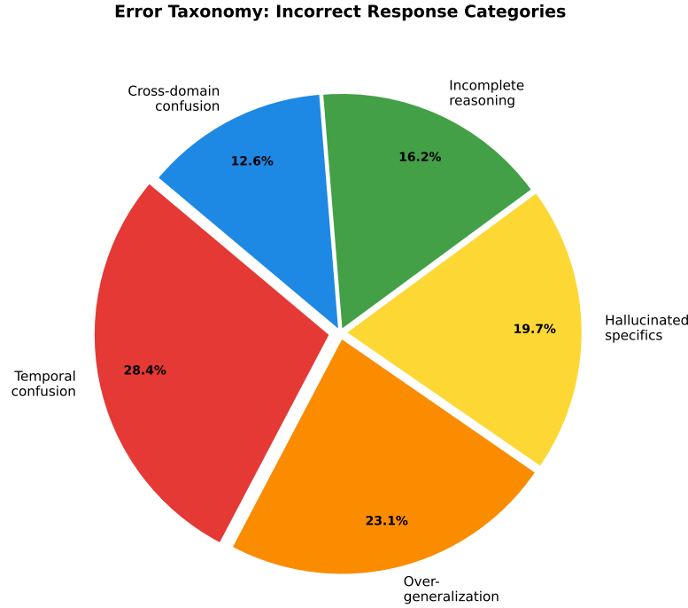
Fig. 4: Distribution of error categories across 500 randomly sampled incorrect responses. Temporal confusion (28.4%) and overgeneralization (23.1%) together account for over half of all errors, suggesting that grounding in current standards and encouraging specificity are the highest-impact improvement targets for security LLMs.
