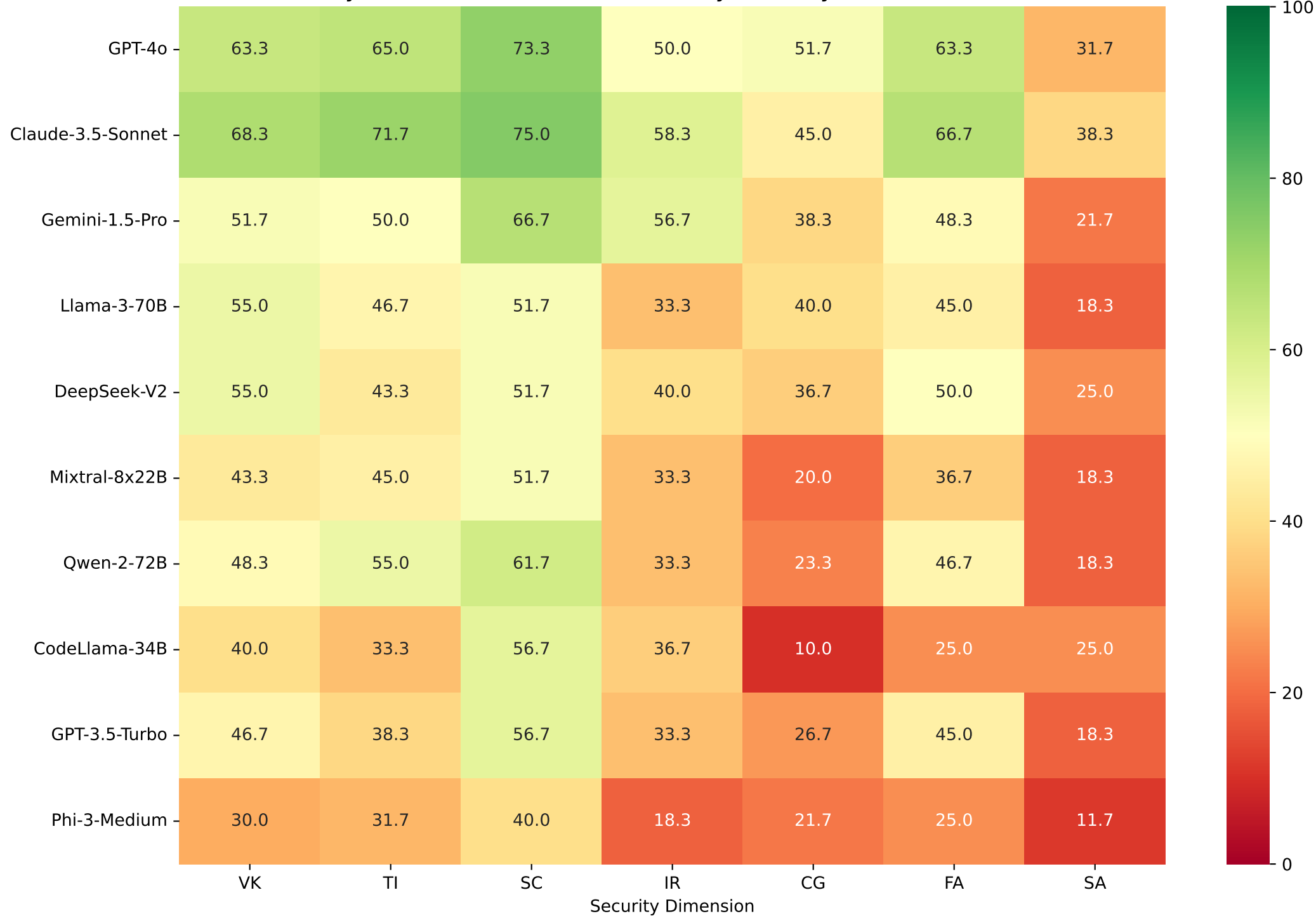
CyberEval: Model Performance by Security Dimension (%)
