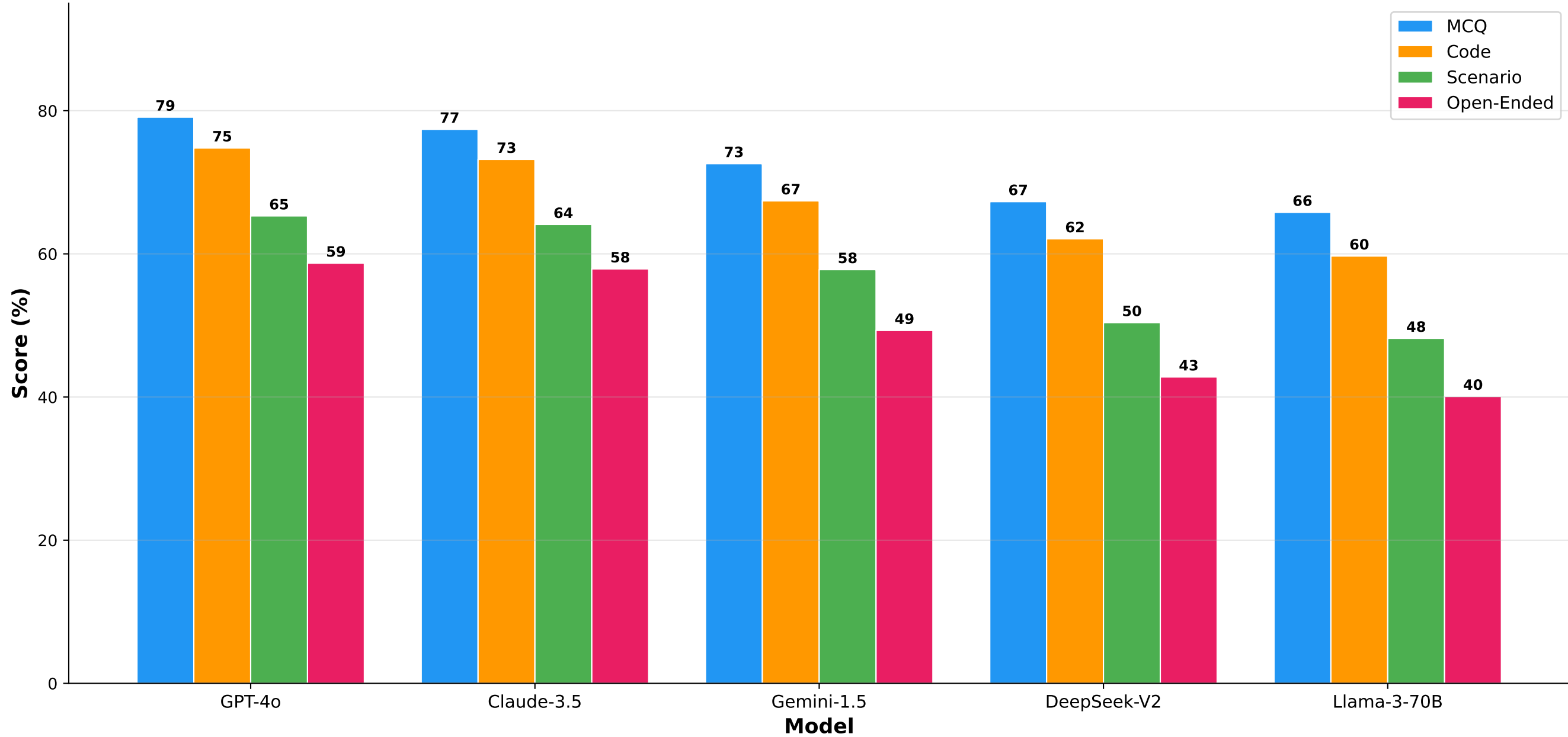
CyberEval Performance by Assessment Format
