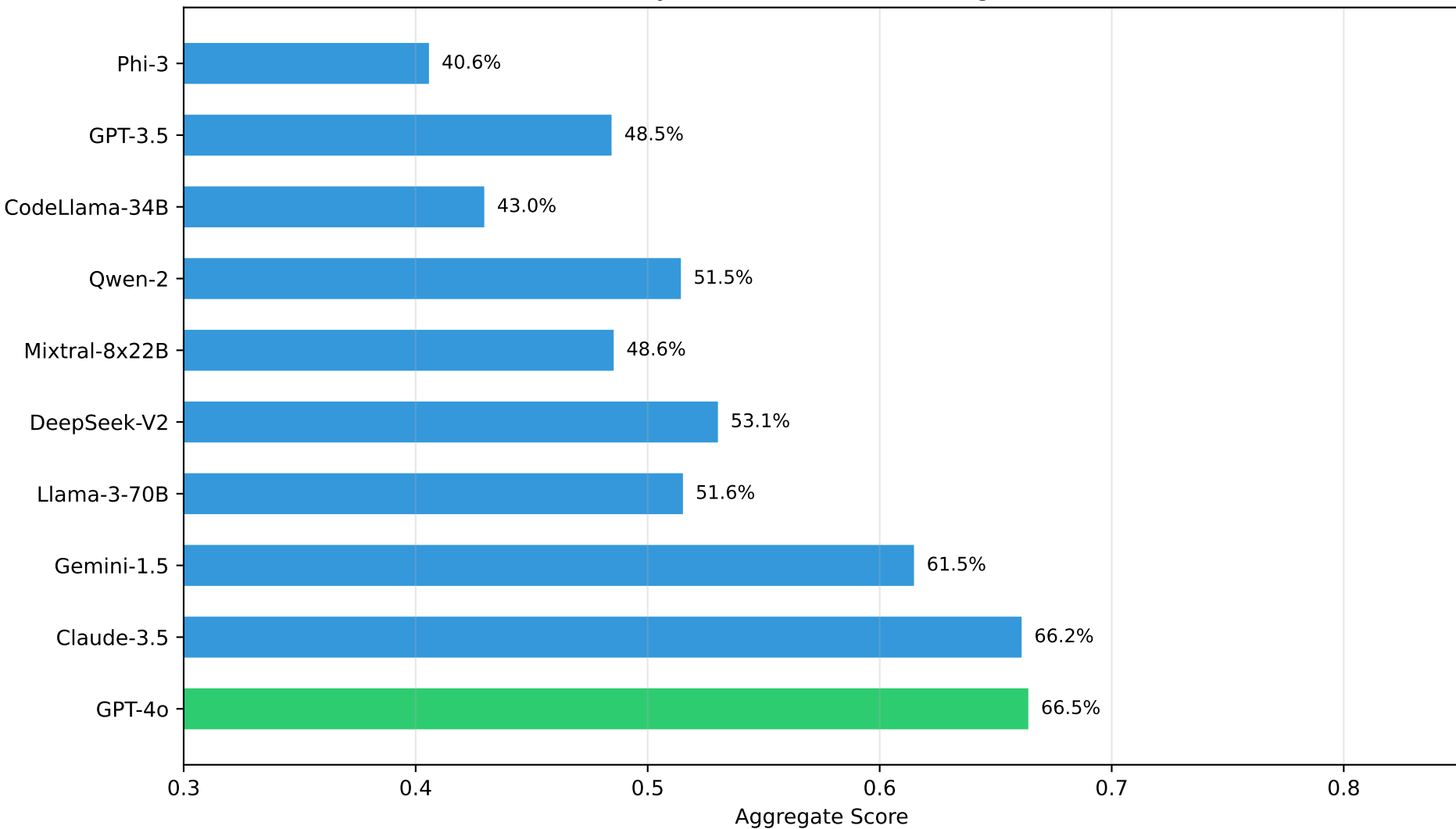
CyberEval: Model Rankings
