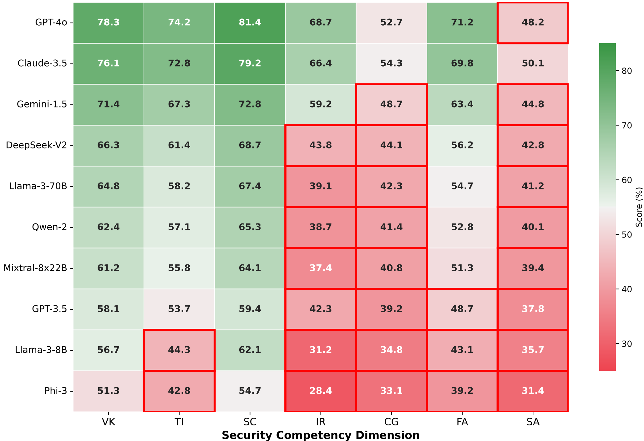
CyberEval: Model Competency Heatmap
