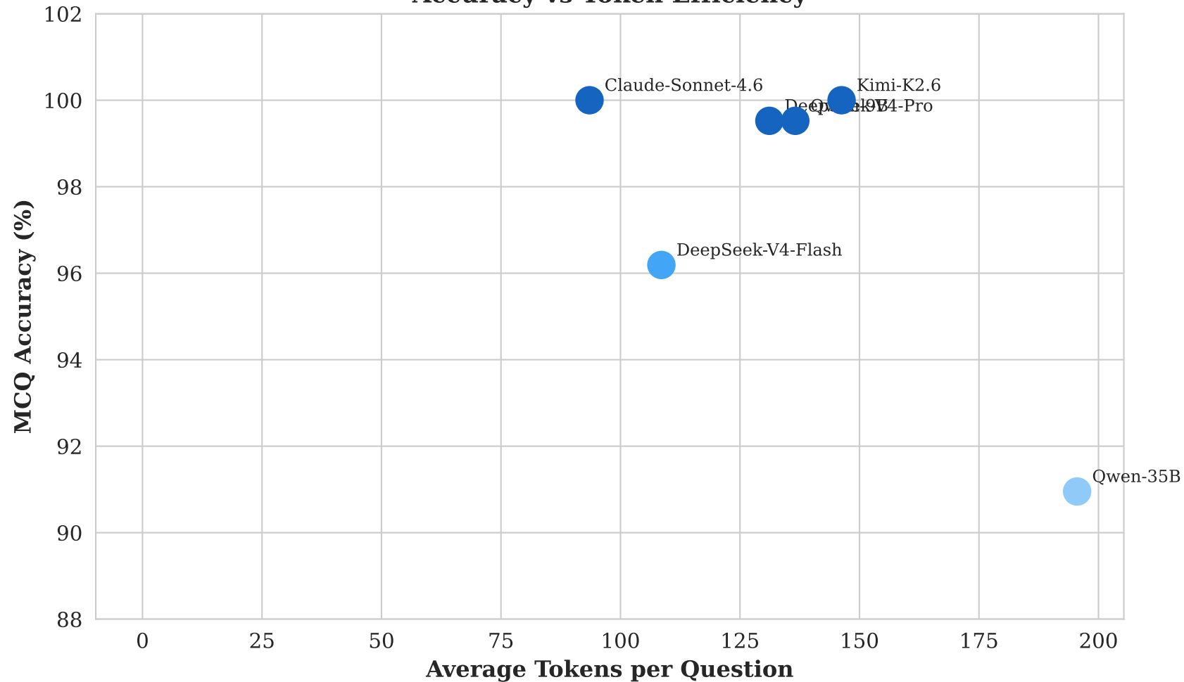
Accuracy vs Token Efficiency
