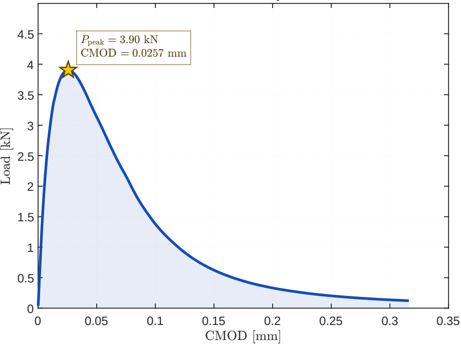
Load--CMOD response
