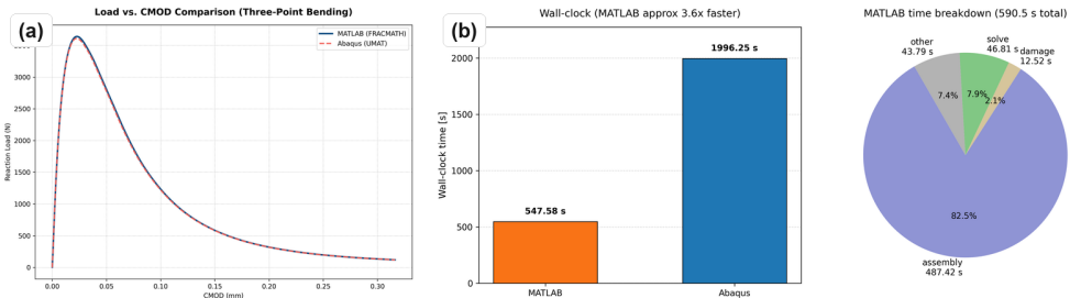
Figure 2: 3PB response and timing: (a) MATLAB and Abaqus load-CMOD response; (b) wall-clock comparison and MATLAB timing breakdown.
