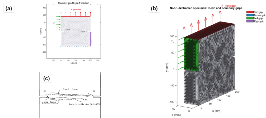
Figure 3: Nooru-Mohamed mixed-mode benchmark: (a) boundary conditions; (b) 3D mesh; (c) experimental crack path from Nooru-Mohamed (Nooru-Mohamed, 1992).
