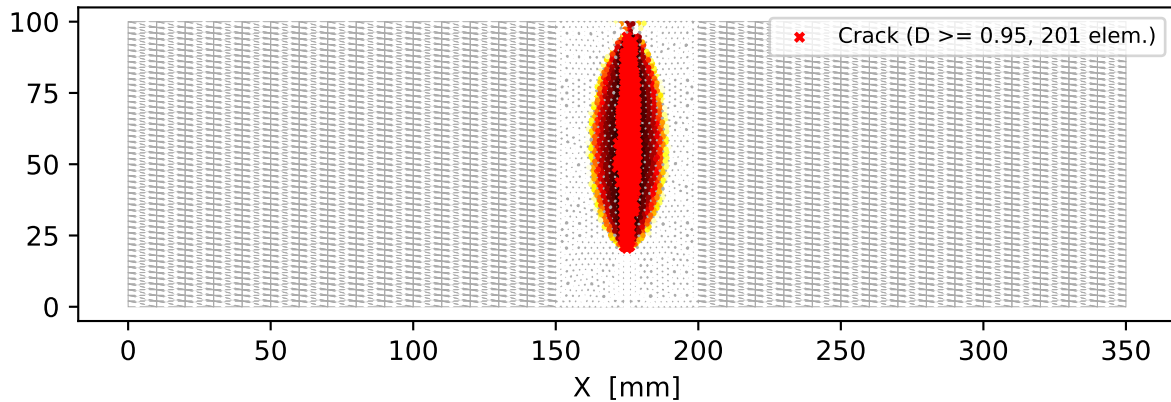
Damage Contour - Undeformed Mesh (Step: Loading | Frame: -1)
