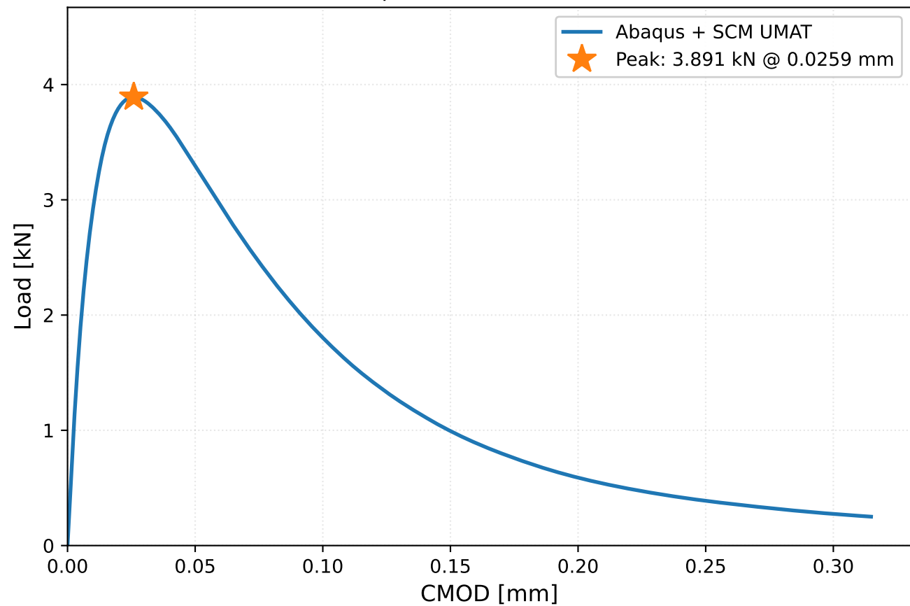
Abaqus 3PB - Load vs CMOD
