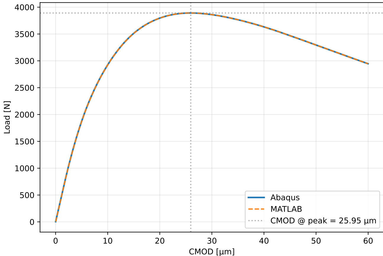
Peak region zoom (CMOD < 60 \mu\text{m} )
