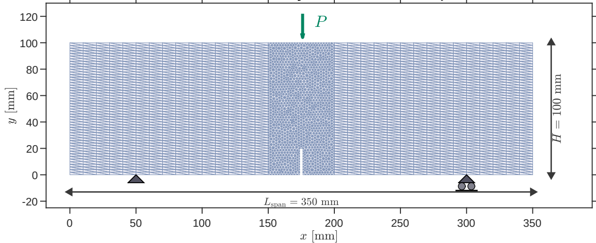
FE mesh — boundary conditions and load point
