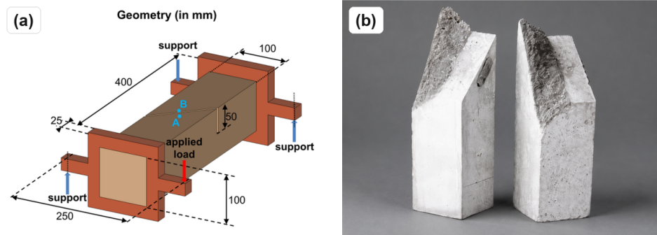
Figure 5: Brokenshire torsion benchmark: geometry and experimental fractured specimen from Jefferson et al. (Jefferson et al., 2004).
