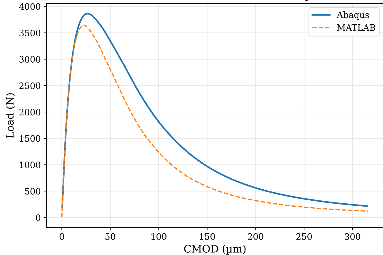
Load vs CMOD — MATLAB vs Abaqus
