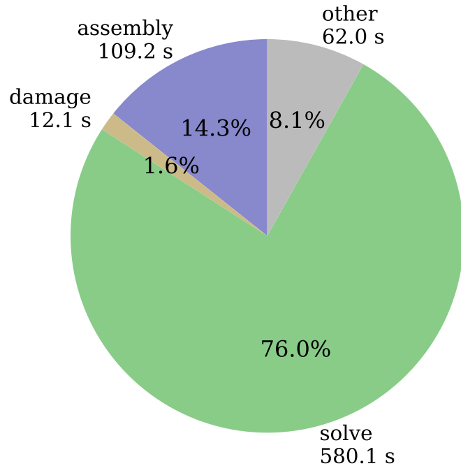
MATLAB time breakdown (763.5 s total)
