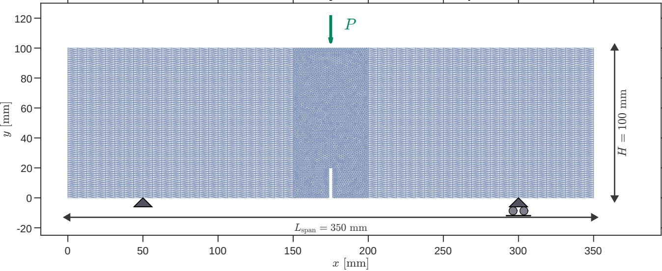
FE mesh — boundary conditions and load point
