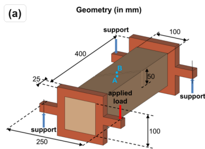
Figure 5: Brokenshire torsion benchmark: geometry and experimental fractured specimen from Jefferson et al. (Jefferson et al., 2004).
