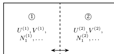
pared-permeable
