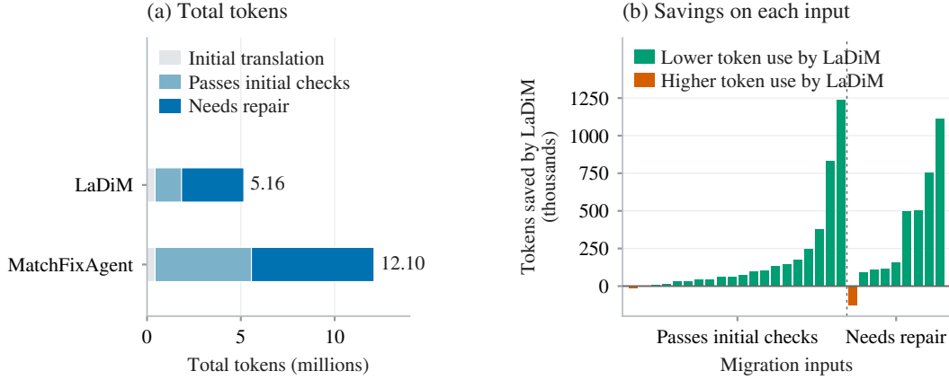
Figure 3: Total and per-input token costs for LaDiM and MatchFixAgent on MindSpore migration. Both accept 50/50 tasks; LaDiM uses 57.4% fewer tokens. (a) Totals include initial translation and subsequent calls grouped by the initial checks. (b) Each bar shows MatchFixAgent tokens minus LaDiM tokens for one distinct source and evaluation input, sorted within each group. Positive values indicate lower LaDiM cost.
