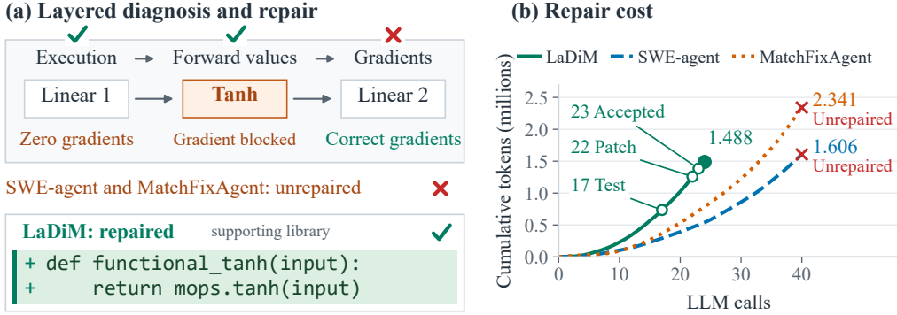
Figure 4: Repairing a silent gradient fault. (a) Layered Diagnosis identifies Tanh as the gradient break. The highlighted code adds its missing MindSpore mapping (registration decorators omitted). (b) Cumulative investigation and repair tokens. LaDiM repairs the program, while both baselines remain unrepaired after 40 calls.
