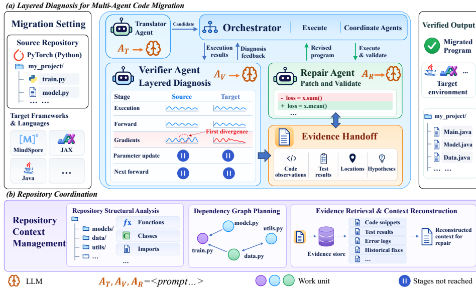
Figure 2: Overview of LaDiM. (a) The Translator Agent produces a candidate, and the Orchestrator executes it, returns measurements, and coordinates the agents. The Verifier Agent applies Layered Diagnosis, comparing source and target in execution, forward values, gradients, and parameter updates. It focuses on the first stage that diverges (gradients in this example), and later stages are marked as not reached. Its code observations, test results, locations, and hypotheses are handed to the Repair Agent, which patches the candidate and submits it for validation. (b) For repositories, repository context management analyzes the repository structure, plans repairs over a dependency graph of work units, and reconstructs the context from an evidence store. A_T , A_V , and A_R are the role instructions of the three agents. The code edit and signal traces are illustrative.
