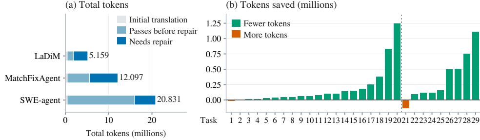
Figure 3: MindSpore migration token costs. (a) Initial translation and subsequent calls, grouped by whether repair is needed. (b) MatchFixAgent minus LaDiM tokens for 29 distinct inputs: tasks 1–20 pass before repair; tasks 21–29 require repair. Savings are sorted within each group.
