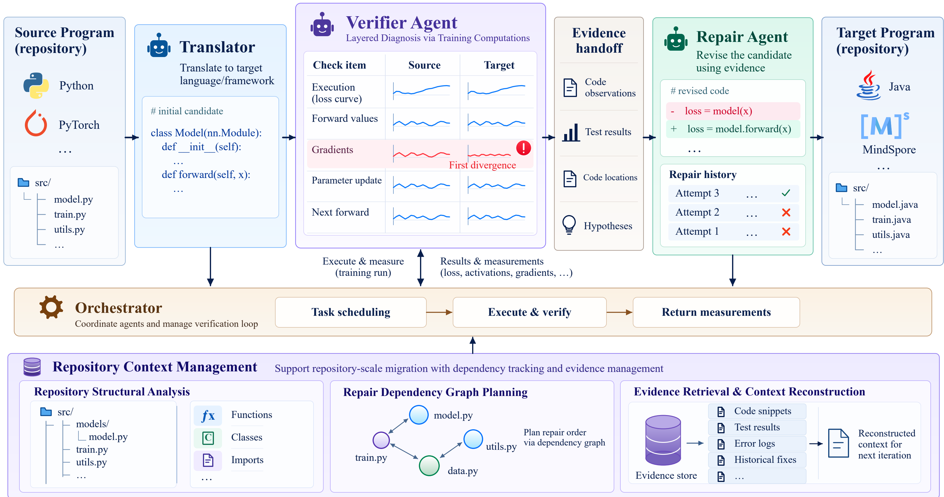
Figure 1: Overview of LaDiM. LaDiM translates, verifies, and iteratively repairs programs with repository context management.
