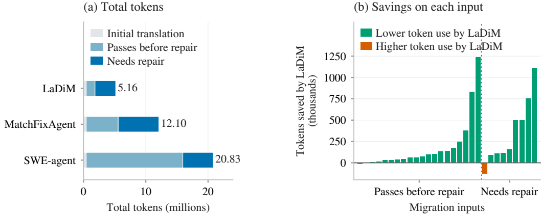
Figure 3: Token costs on MindSpore migration. (a) Total tokens for LaDiM, MatchFixAgent, and SWE-agent are divided into initial translation and subsequent calls for programs that pass or fail their first evaluation before repair. The latter costs are labeled Passes before repair and Needs repair . (b) Each bar shows MatchFixAgent tokens minus LaDiM tokens for one distinct combination of source program and evaluation requirements, sorted by increasing difference within each group. LaDiM and MatchFixAgent both accept 50/50 tasks. LaDiM uses 57.4% fewer tokens. Positive values indicate lower LaDiM cost.
