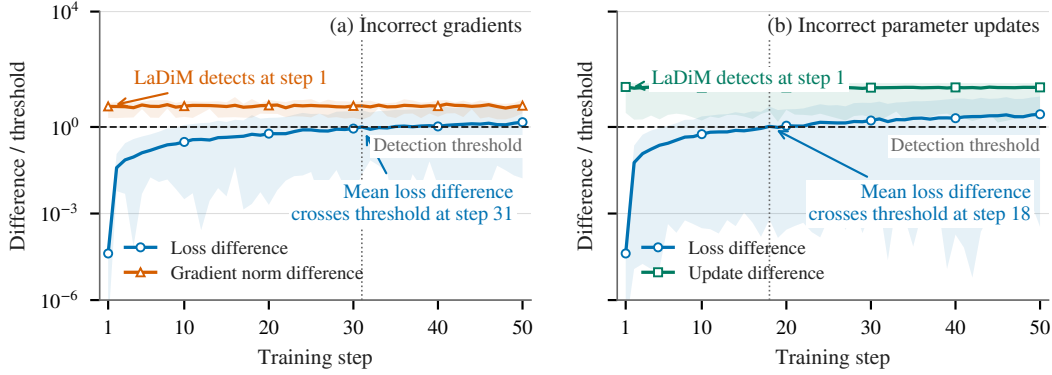
Figure 4: Training signal detection and loss difference threshold crossings. Each panel contains 12 runs from four models and three seeds. LaDiM detects gradient scaling (a) and partial update suppression (b) at step 1 in every run. The mean loss difference crosses its threshold at step 31 in (a) and step 18 in (b). Within 50 training steps, the loss difference exceeds its threshold in 3 of 12 runs with gradient errors and 4 of 12 runs with update errors. Differences are divided by their detection thresholds. Curves show means, and shading spans the minimum and maximum across runs.
