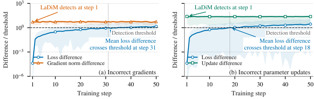
Figure 5: Detection of (a) gradient scaling and (b) partial update suppression over 50 training steps. Solid lines show the mean over 12 runs (four models \times three seeds), and shaded bands show the minimum and maximum across these runs at each step. Each difference is divided by its detection threshold, so values above the dashed line count as detected. Gradient and update checks detect both faults at step 1 in every run; with the loss threshold of 0.02, the mean loss difference first crosses at steps 31 and 18, respectively.
