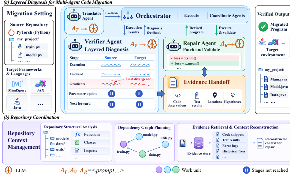
Figure 2: Overview of LaDiM. (a) The Translator produces a candidate, and the Orchestrator compares its execution, forward values, gradients, and parameter updates with the source. The Verifier investigates the first divergent stage (gradients here) and hands code observations, test results, locations, and hypotheses to the Repair Agent. The Repair Agent tests and edits the candidate, using the Orchestrator’s feedback until acceptance or budget exhaustion. (b) Repository context management analyzes code structure, orders repairs through work-unit dependencies, and reconstructs compact contexts from archived evidence.
