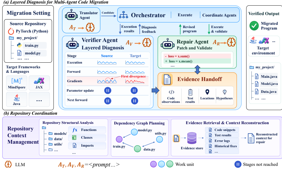
Figure 2: Overview of LaDiM. (a) The Translator Agent produces an initial candidate, and the Orchestrator executes it alongside the source program to measure execution, forward values, gradients, and parameter updates. If the candidate is not accepted, the Verifier Agent applies Layered Diagnosis: it compares these stages in training order and investigates the first one that diverges (gradients in this example), so later stages are not reached. Its code observations, test results, code locations, and hypotheses are handed to the Repair Agent, which tests and edits the candidate and submits it to the Orchestrator. The Orchestrator returns the remaining discrepancies to the Repair Agent until the candidate is accepted or the budget is exhausted. (b) For repositories, repository context management analyzes the repository structure, orders repairs over a dependency graph of work units, and stores evidence outside the conversation so that a compact context can be reconstructed when the agent switches units.
