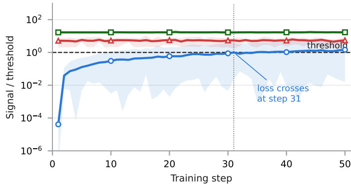
(a) Gradient computed incorrectly
