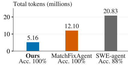
Figure 1: Tokens used on 50 PyTorch to MindSpore migrations tasks.
