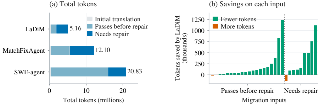
Figure 3: Token costs on MindSpore migration. (a) Costs comprise initial translation and subsequent calls, grouped by whether programs pass evaluation before repair. (b) Tokens saved by LaDiM compared to MatchFixAgent, sorted from low to high within each group. Both methods accept 50/50 tasks, while LaDiM uses significantly fewer tokens.
