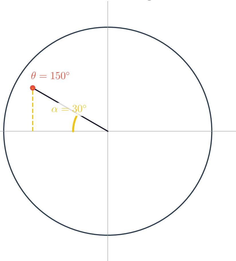
Reference Angle
