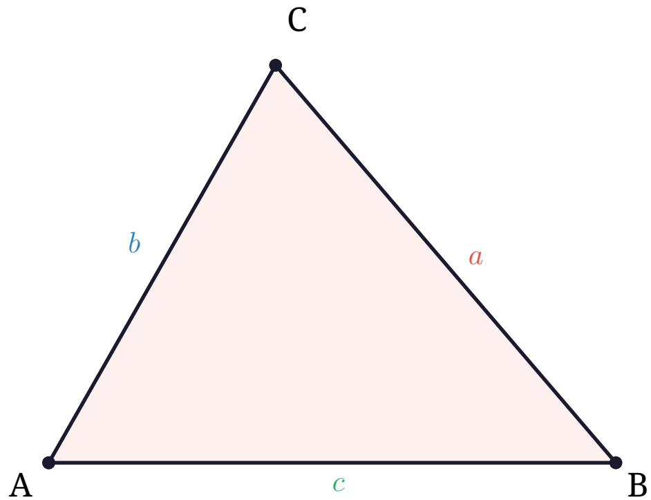
Law of Sines
