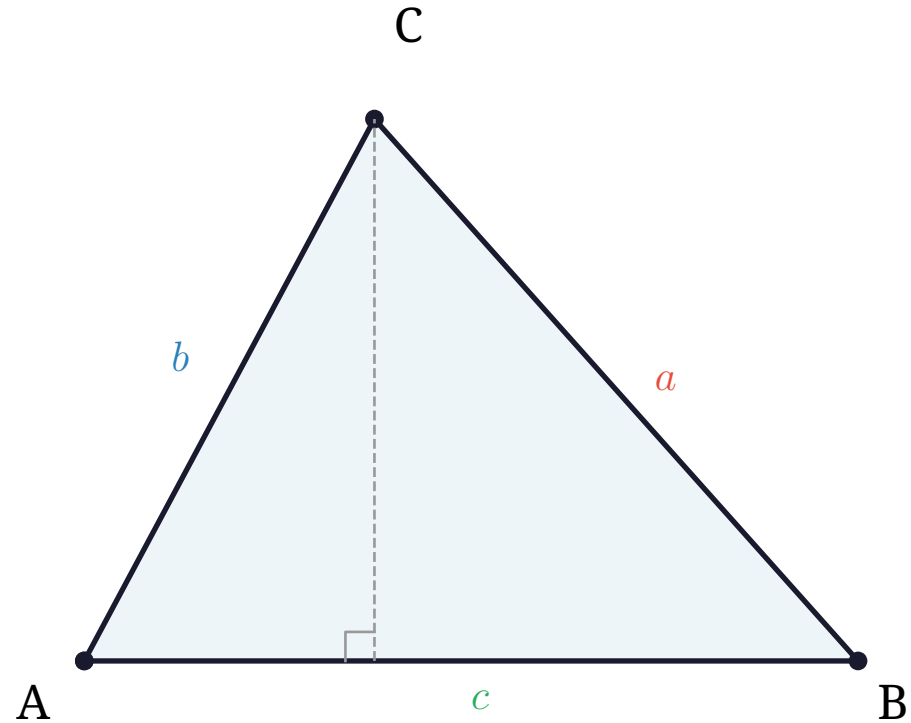
Law of Cosines
