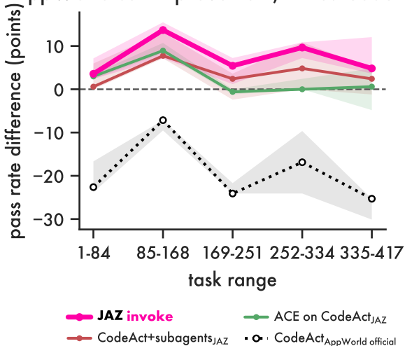
AppWorld self-improvement, minus CodeAct
