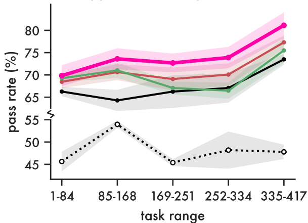
AppWorld self-improvement
